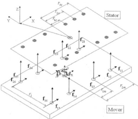
Fig. 6 Free body diagram of mover
