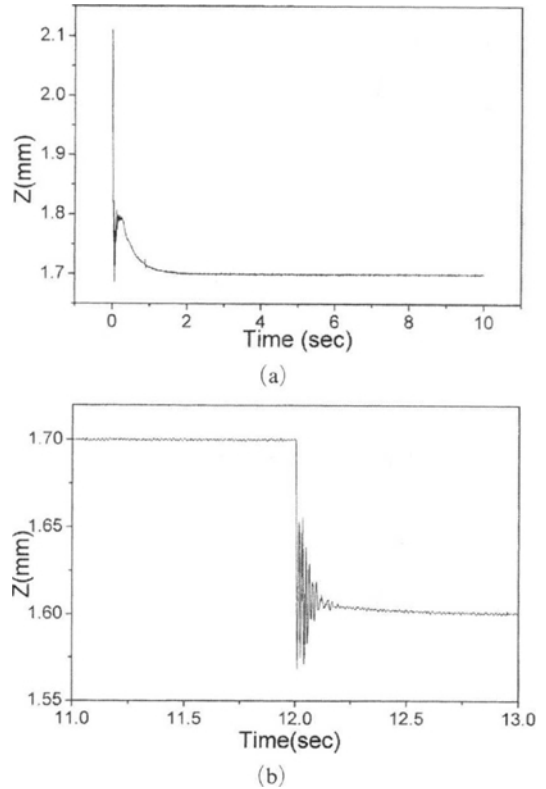
Fig. 8 Experimental results (a) suspension test (b) step response (100 \mu\text{m} )
