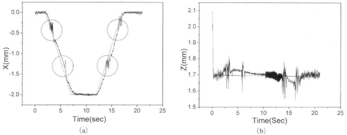
Fig. 9 Trapezoidal linear motion test results (a) horizontal result (b) vertical result
